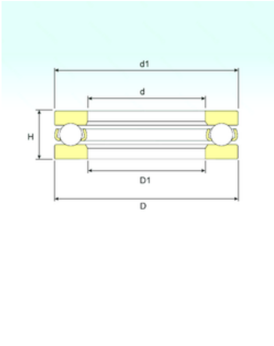
51215 Bearing 2D drawings and 3D CAD models
